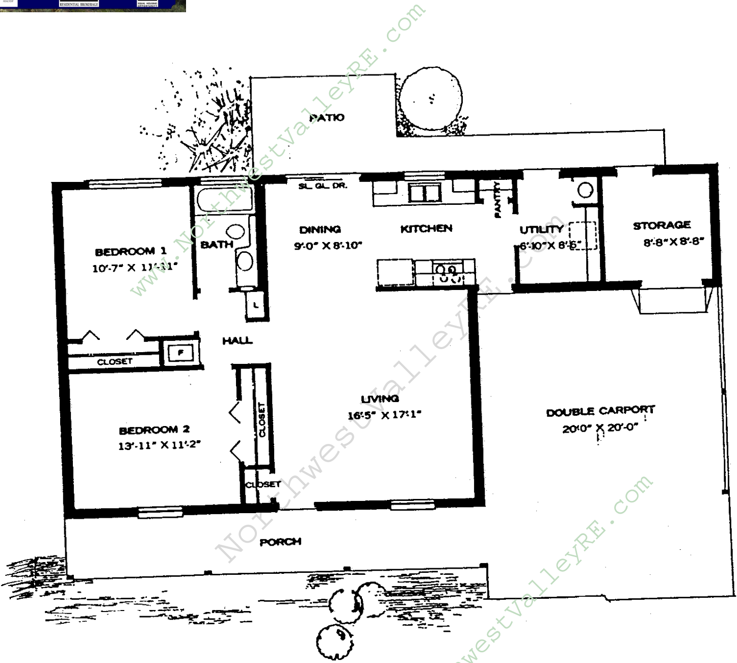
PLAN 51 DOUBLE CARPORT SUN CITY, ARIZONA 11-1-86
