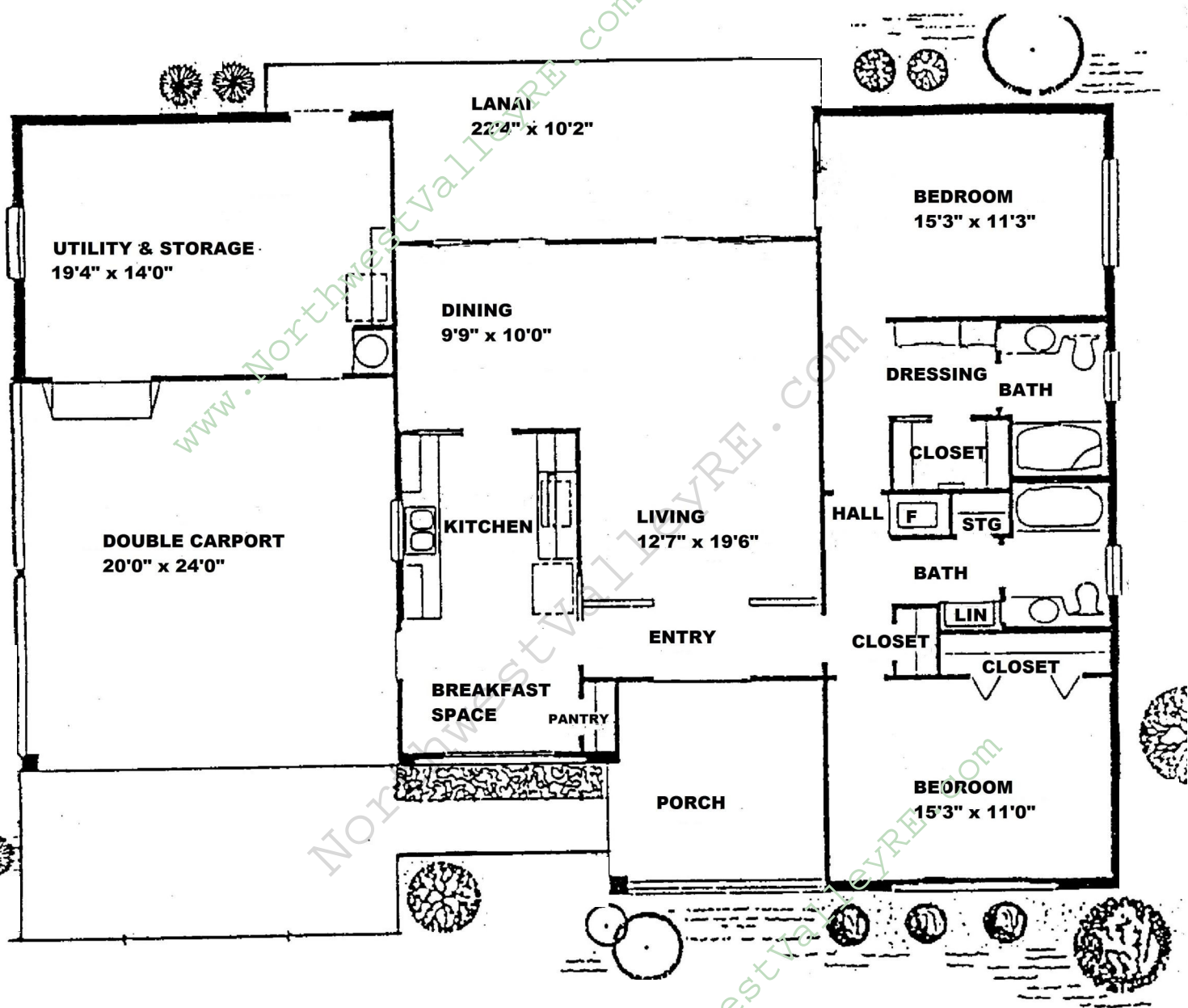
Plan H63 1,326 Square Feet
