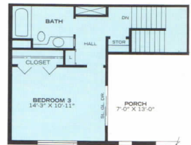
Plan M-5 Alternate Second Story
